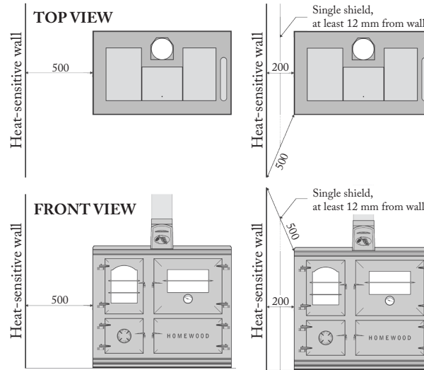
Figure D: Single Shield Example
