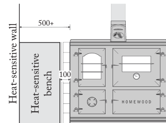
Figure E: Double Shield Example
